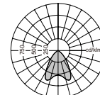
Standard beam
