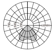
Wide Beam(95°)
